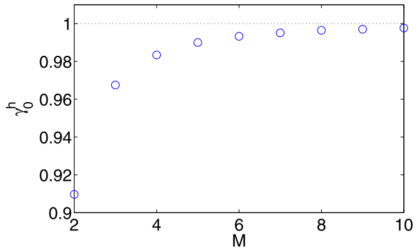
Fig. 9 (Color online) The extrapolated smallest eigenvalue \gamma_0^h as a function of the number M of annuli shown on Fig. 5d, with hS_A = \pi and \delta \rightarrow 0
