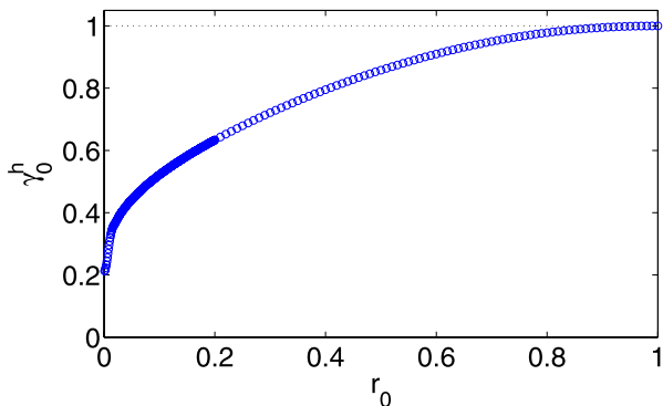
Fig. 7 (Color online) The extrapolated smallest eigenvalue \gamma_0^h as a function of the radius r_0 of the reactive region (the disk) shown on Fig. 5a, with hS_A = \pi
