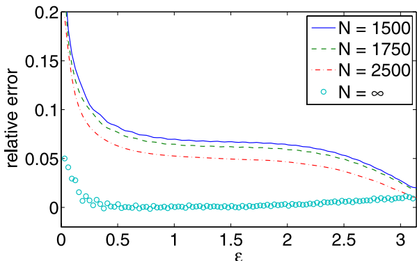
Fig. 10 (Color online) The relative error between the exact formula (16) and the truncated spectral representation (17) for the mean exit time from the unit disk whose boundary is reflecting but for an absorbing arc of length 2\varepsilon
