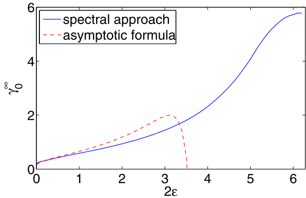
Fig. 11 (Color online) The smallest eigenvalue \gamma_0^\infty for the unit disk when the reactive region is an arc of length 2\varepsilon (with h = 10^8 ). When 2\varepsilon goes to 2\pi (the whole circle), \gamma_0^\infty approaches the theoretical value 5.7829\dots , as expected. The asymptotic formula (18) is accurate for small \varepsilon but inapplicable for large \varepsilon
