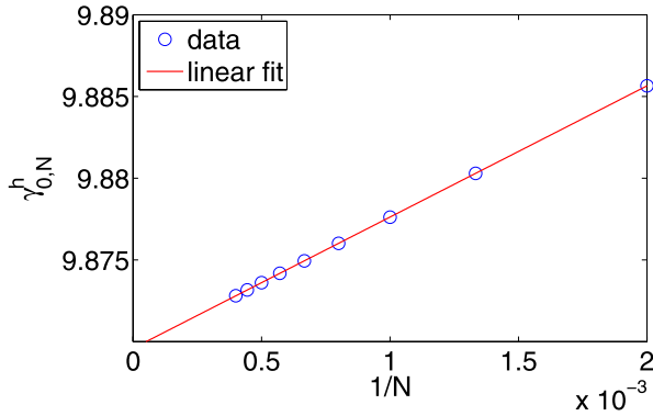
Fig. 1 (Color online) The smallest eigenvalue \gamma_{0,N}^h of the truncated matrix \Lambda + h\mathcal{B} (of size N \times N ) for \Omega = (0, 1) , A = \{0, 1\} , h = 10^8 . The error is almost linear with 1/N
