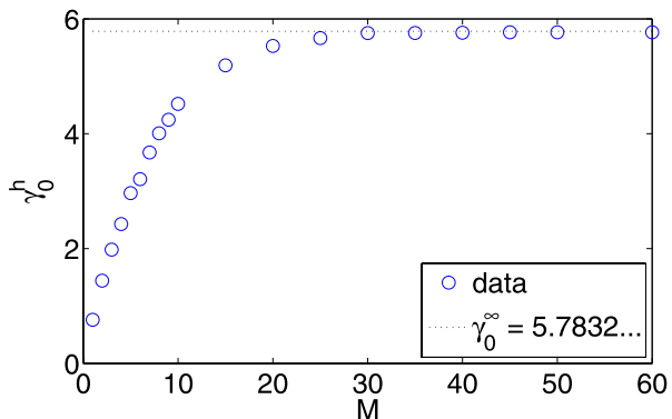
Fig. 6 (Color online) The extrapolated smallest eigenvalue \gamma_0^h for the unit disk, when A is composed of M identical arcs of the unit circle. The total length L is kept to be 2\pi/5 for different M , and h = 10^8 . When M increases, the eigenvalue \gamma_0^h rapidly approaches the limit 5.7832... which corresponds to a perfectly reactive circle (cf. Fig. 3)
