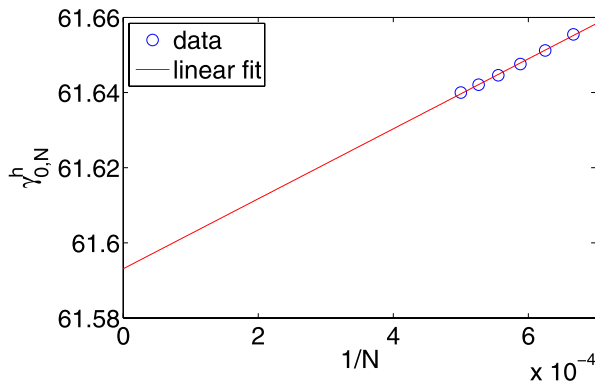
Fig. 2 (Color online) The smallest eigenvalue \gamma_{0,N}^h of the truncated matrix \Lambda + h\mathcal{B} (of size N \times N ) for \Omega = (0, 1) , A = [0.2, 0.8] , h = 10^8 . The error is approximately linear with 1/N
