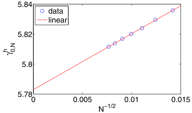
Fig. 3 (Color online) The smallest eigenvalue \gamma_{0,N}^h of the truncated matrix \Lambda + h\mathcal{B} (of size N \times N ) for the unit disk, when \Lambda is the unit circle, and h = 10^8 . The error is almost linear with 1/\sqrt{N}
