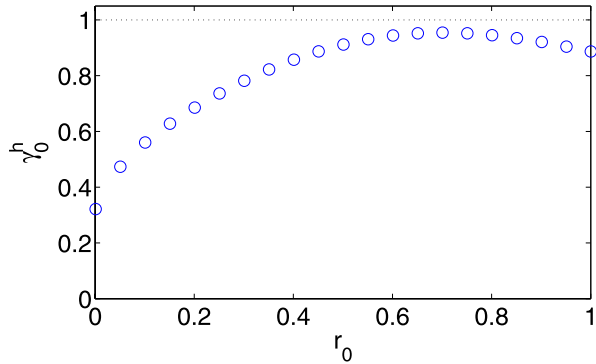
Fig. 8 (Color online) The extrapolated smallest eigenvalue \gamma_0^h as a function of the radius r_0 of the reactive region (the annulus of width \delta ) shown on Fig. 5c, with hS_A = \pi and \delta \rightarrow 0
