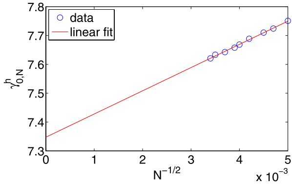
Fig. 4 (Color online) The smallest eigenvalue \gamma_{0,N}^h of the truncated matrix \Lambda + h\mathcal{B} (of size N \times N ) for the unit disk, when A is a smaller disk of radius r_0 = 0.5 , and h = 10^8 . The error is approximately linear with 1/\sqrt{N}
